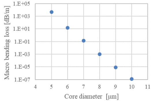
Fig. 2 Macro bending loss for various core diameter of SMF
