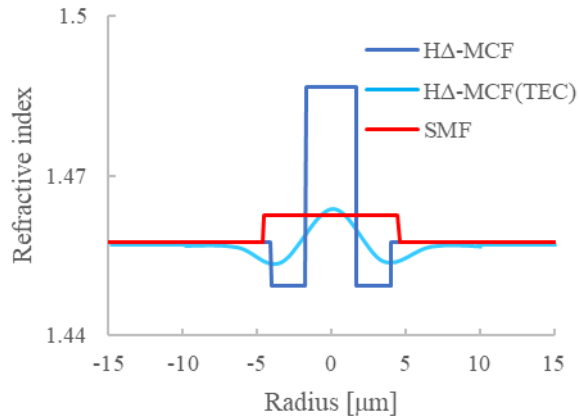
Fig. 3(b) Refractive index profile of HA-MCF after stretching.
