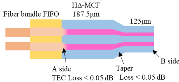
Fig. 1 Structure of narrow pitch FIFO
