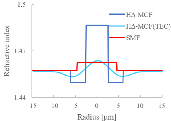
Fig. 3(a) Refractive index profile of HA-MCF
