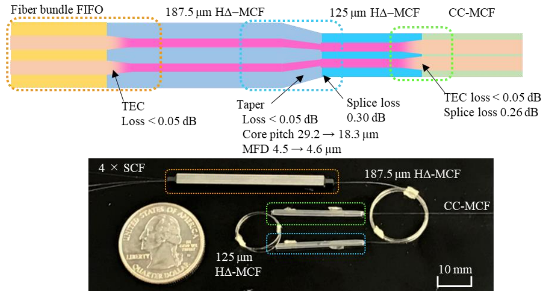
Fig. 4 Structure of narrow pitch FIFO
